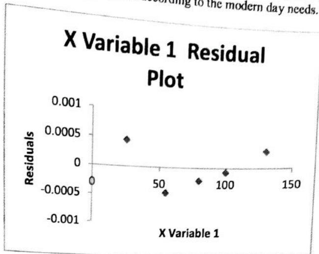
Fig.8. Residual Plot
